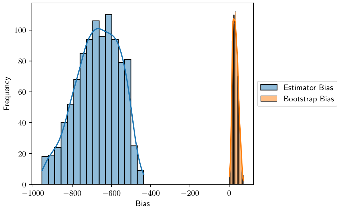
Distribution of Bias_Brain_Cerebellum
